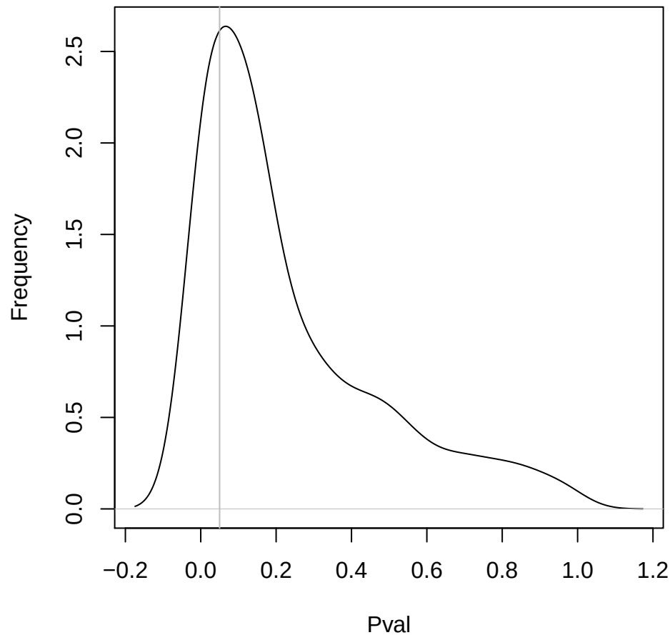
CoopBreed Interval.final Brownie pvals , # sims = 500 Mean = 0.2312 / StdDev = 0.2421
